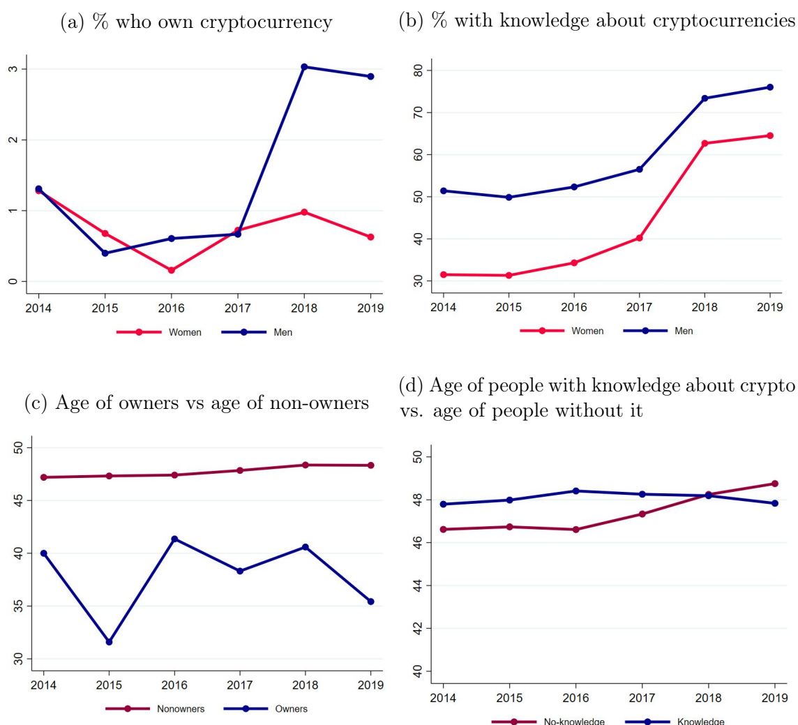
Figure 8: Cryptocurrency trends (2014-19).
